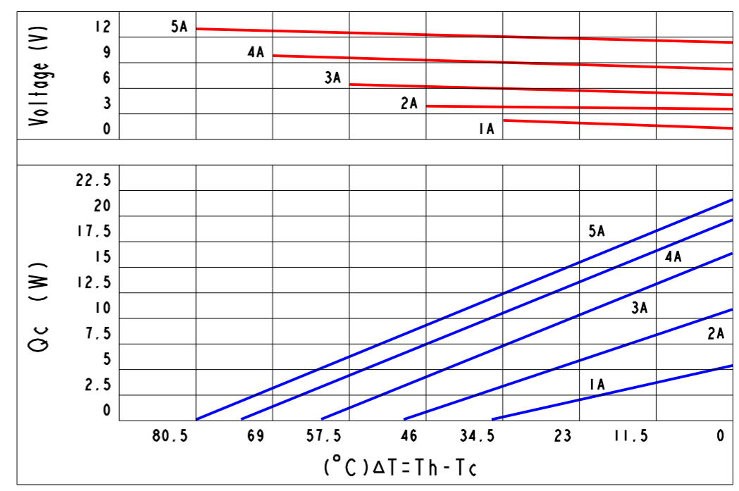
Curve Chart(Be Confined To TEC2-148055025):
